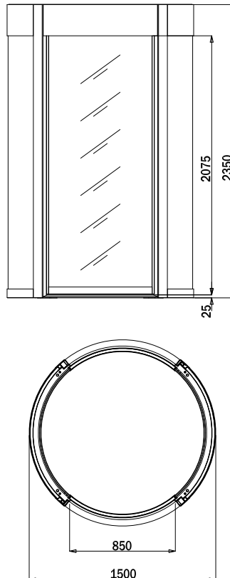
CYLINDRICAL SECUREDOOR VARIANT
