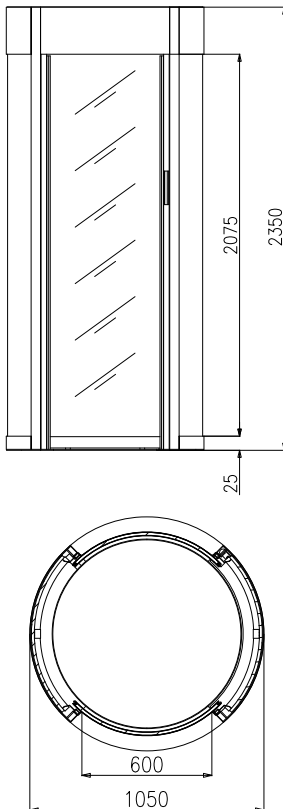
STANDARD CYLINDRICAL SECUREDOOR
